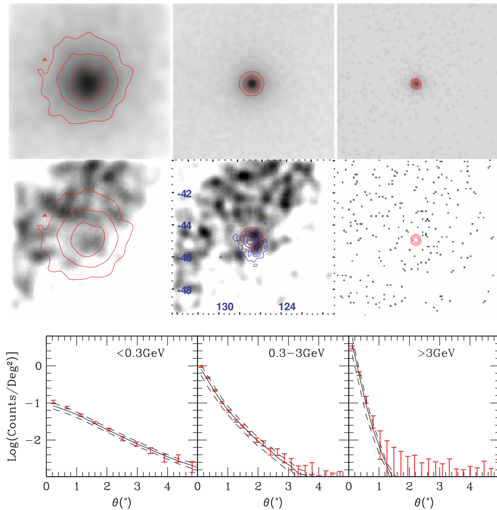
Figure 4. On- ( \phi = 0.05\text{--}0.65 , top row) and off- ( \phi = 0.65\text{--}1.05 , middle row) pulse phase images in three energy bands. Each panel spans 10^{\circ} \times 10^{\circ} in equatorial coordinates centered on Vela (R.A. and decl. marked in degrees in the central panel). On-pulse data are dominated by the point source; the panels have a hard square root stretch to show the faint wings of the PSF. The off-pulse images (linear grayscale) are dominated by Galactic diffuse emission; some of the structure is due to limited count statistics. Contours of the point source at 0.5, 0.25, and 0.125 of the peak intensity are shown (red) in each frame. In the middle energy off-pulse image, we also show the HESS Vela PWN contours (Aharonian et al. 2006; blue). Along the bottom row, background-subtracted Vela PSFs (red error bars give the statistical error in the observed counts) are compared with simulations based on prelaunch descriptions of expected LAT performance (solid lines) and estimates of the systematic uncertainty in the model PSF (dashed lines).
