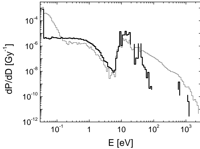
Fig 4: Histogram of energy transfers for C[10MeV/n] irradiation. Thin line: energy transferred to the 10x10x10 nm 3 cubes of a 10x10x10 μm 3 sample irradiated at a dose of 1 Gray. Thick line: energy of the individual events generated by the irradiation. This latter curve was arbitrarily normalized for the sake of easy comparison.
