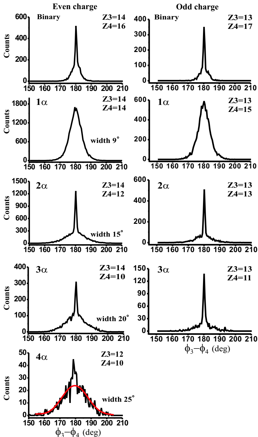
FIG. 13: (Color online) Yields, N(Z_3, Z_4) , of coincident fragments with charges indicated by Z_3+Z_4 , as a function of the out-of-plane angles ( \phi_3 - \phi_4 ) (in degrees). The width (FWHM) of the angular correlations for the different fission channels are shown.
