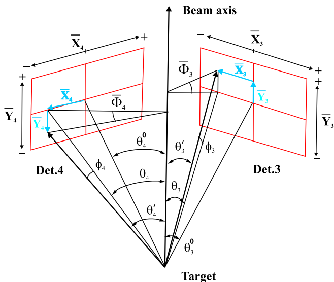
FIG. 3: (Color online) Definitions of the in-plane (\theta_3, \theta_4) and out-of-plane (\phi_3, \phi_4) scattering angles obtained from the \bar{X} and \bar{Y} read-outs of the position sensitive detectors.
