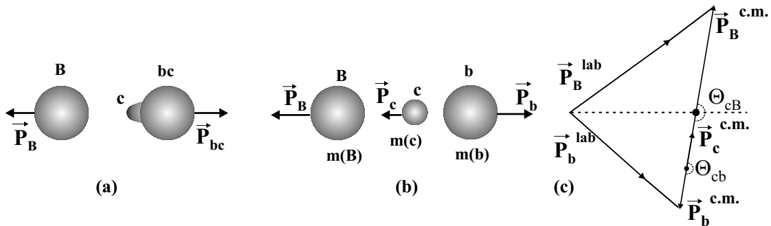
FIG. 23: Sequential fission decay: Ternary fission as a consecutive fast two-step process. The first step - (a), a binary decay of the hyper deformed compound system in two fragments B + (b + c) . The second step - (b) - the decay of (b + c) , cluster C emission from one of the fragments, (c) the vectors in the laboratory and the centre of mass systems. The configuration is assumed to be collinear at high angular momentum.
