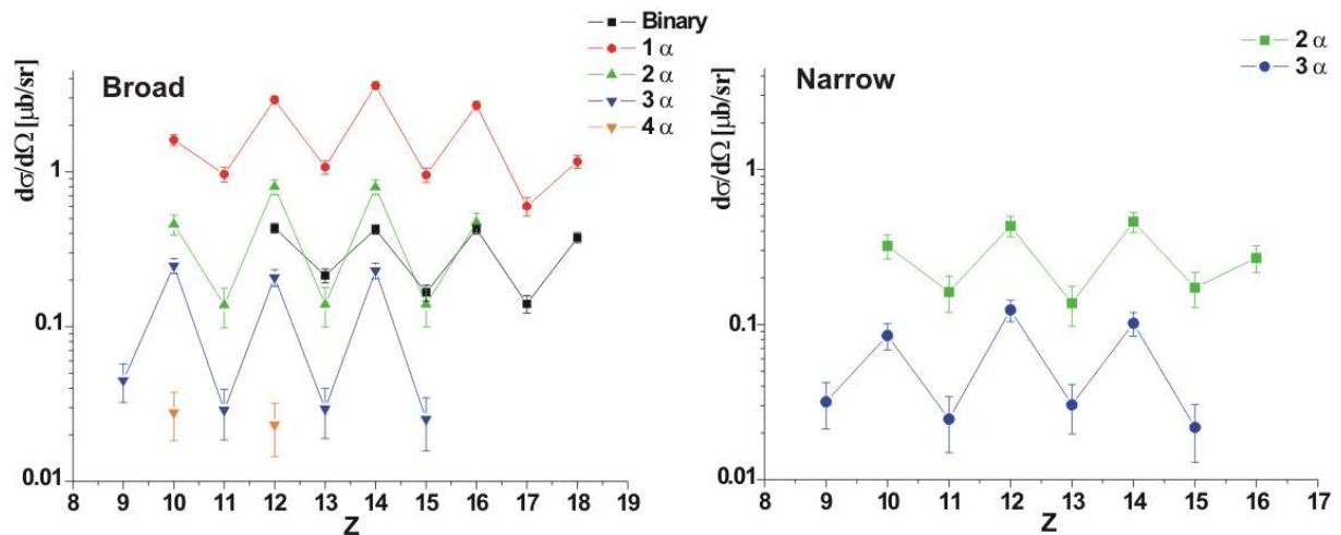
FIG. 20: (Color online) Differential cross sections in the reaction ^{36}\text{Ar} + ^{24}\text{Mg} for channels defined by (Z_3+Z_4+\alpha) of the broad (binary) and narrow (ternary) components of the coincident fission fragments. They represent the average over the angular range between \theta_{c.m.} = 65^\circ to 120^\circ in the centre-of-mass system. The fission channels with missing 1\alpha , 2\alpha , 3\alpha and 4\alpha -particles are shown.
