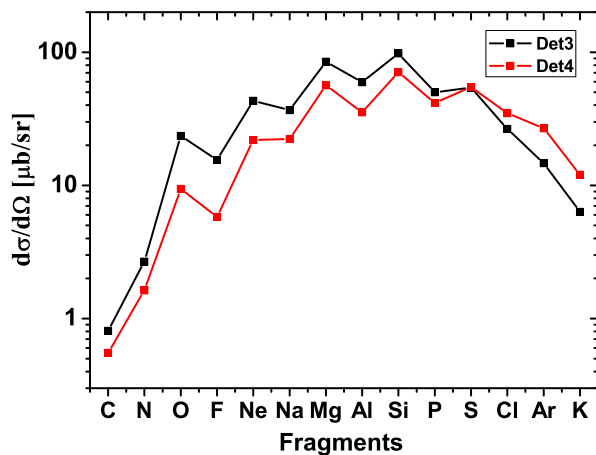
FIG. 7: (Color online) Inclusive coincidence yields, obtained with a gate set for Z-identification in either of the detectors (3) or (4) for the reaction ^{36}\text{Ar}+^{24}\text{Mg}\rightarrow Z_3+x or Z_4+x , for an angular range of \theta_{c.m.} = 65^\circ - 120^\circ .
