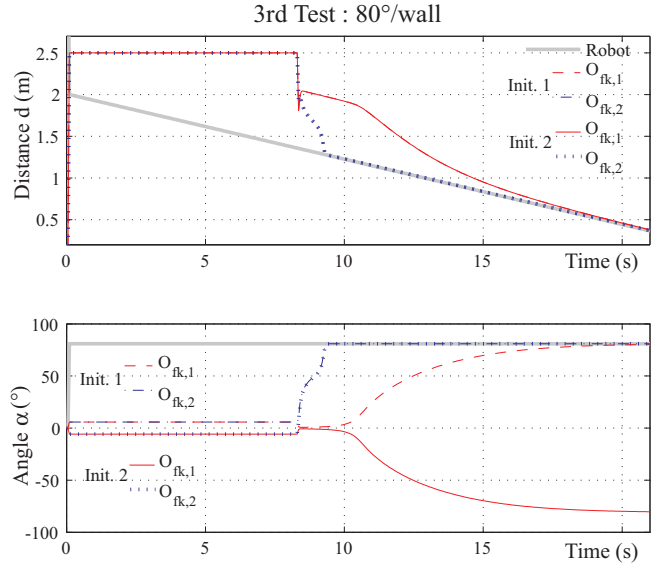
Fig. 11. Third test 80^\circ /wall. Observers O_{fk,1} and O_{fk,2} . Estimation results of wall position d and angle \alpha .
