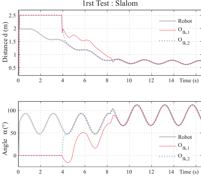
Fig. 9. Slalom test. Observers O_{fk,1} and O_{fk,2} . Estimation results of wall position d and angle \alpha .
