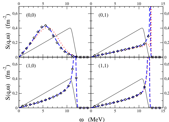
FIG. 2: (Color online) RPA Strength function (open diamonds) compared with continuous fraction approximation (1st order: dotted line, 2nd order: dashed line) calculated with Gogny D1 interaction in symmetric nuclear matter, at saturation density \rho_0 and momentum transfer q=27 MeV. The thin lines represent the uncorrelated HF strengths.
