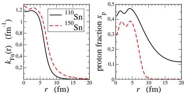
FIG. 7: (Color online) The neutron Fermi momentum and the proton fraction, obtained with the HFB densities, for two mid-shell Sn nuclei, ^{110}\text{Sn} (the solid line) and ^{150}\text{Sn} (the dashed line).
