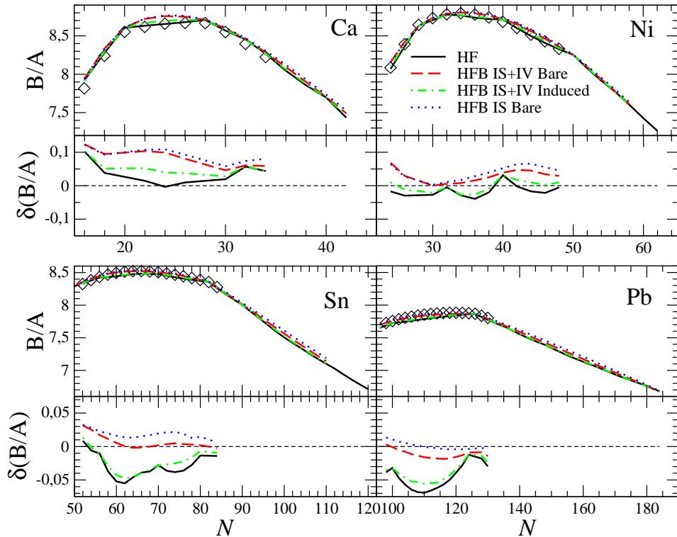
FIG. 2: (Color online) Comparison of the HFB calculations with the experimental binding energies, B/A . The solid line shows the results without pairing interaction (HF), while the dotted, short dashed, and long dashed lines are obtained with the pairing interactions IS+IV Bare, IS+IV Induced and IS Bare, respectively. For each isotopic chain, we also plot the difference \delta(B/A) = B(\text{th.})/A - B(\text{exp.})/A between the theoretical and the experimental values for the binding energy. All units are given in MeV. See the text for more details.
