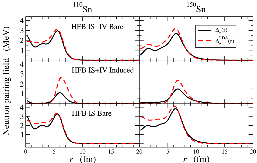
FIG. 8: (Color online) Comparison of the pairing field \Delta_n^{LDA}(r) in the local density approximation (the dashed line) with that of the HFB calculations (the solid line) for the ^{110}\text{Sn} and ^{150}\text{Sn} nuclei. The pairing fields obtained with the different pairing interactions, IS+IV Bare, IS+IV Induced and IS Bare, are plotted separately.
