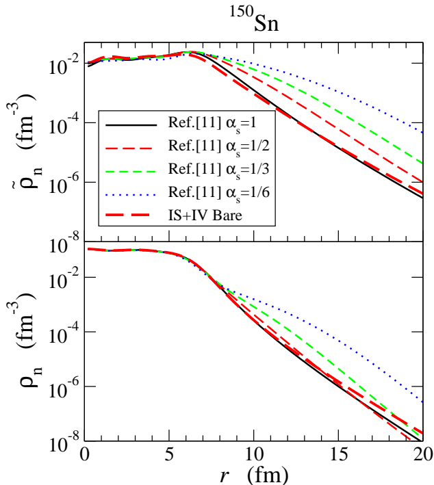
FIG. 6: (Color online) Comparison of particle and pairing densities for the nucleus ^{150}\text{Sn} obtained with several sets of interaction in Ref. [11] and with the IS+IV Bare interaction. See the text for more details.
