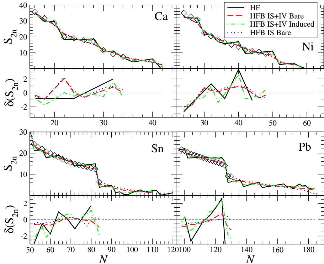
FIG. 3: (Color online) Comparison between HFB and experiments for the two-neutron separation energies S_{2n} . The value \delta(S_{2n}) is defined as \delta(S_{2n}) = S_{2n}(\text{th.}) - S_{2n}(\text{exp.}) . See the caption of Fig. 2 and the text for details.
