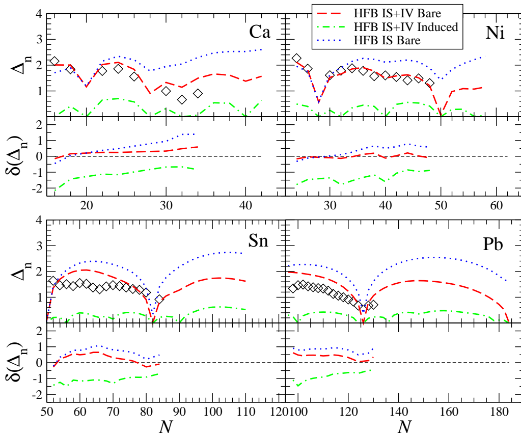
FIG. 4: (Color online) Comparison of the HFB pairing gaps \Delta_n calculated with Eq. (10) with the OES given by \Delta^{(3)} . The value \delta(\Delta_n) is defined as \delta(\Delta_n) = \Delta_n(\text{th.}) - \Delta_n(\text{exp.}) . See the caption of Fig. 2 and the text for details.
