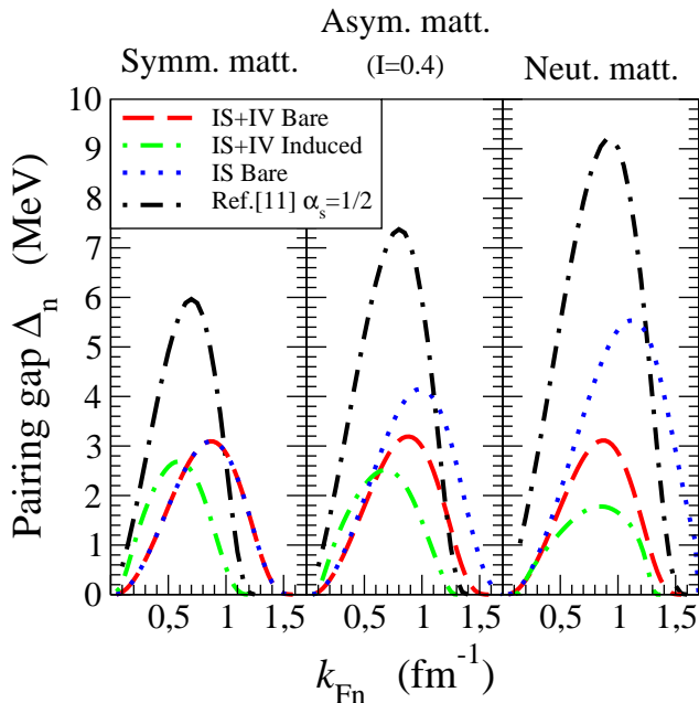
FIG. 5: (Color online) Pairing gaps in uniform matter obtained from the solution of the BCS equations with the pairing interactions IS+IV Bare, IS+IV Induced, IS Bare and the isoscalar interaction of Ref. [11] with \alpha_s = 1/2 and \eta_s = 1 . Notice that the results of IS+IV Bare is identical to those of IS Bare in symmetric matter. See the text for more details.
