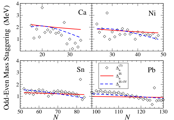
FIG. 1: (Color online) The experimental odd-even mass staggering \Delta_n^{(3)} given by Eq. (9) for the semi-magic Ca, Ni, Sn and Pb isotopes. It is compared with the phenomenological fits \Delta_n^{\text{IS}} = 13.3/A^{1/2} \text{ MeV} and \Delta_n^{\text{IS+IV}} = [7.2 - 44(1 - 2Z/A)^2]/A^{1/3} \text{ MeV} proposed in Ref. [28].
