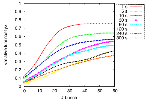
Figure 3: Beam-based IP position feedback simulation for the e^+e^- collision with ground motion model B applied for successive time intervals along the BDS. The average relative luminosity is calculated over 50 seeds.
