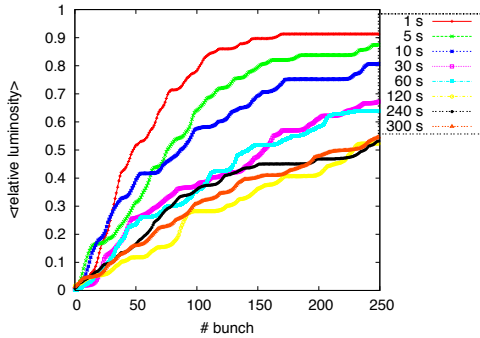
Figure 5: Beam-based IP position and IP angle feedback simulation for the e^-e^- collision with ground motion model B applied for successive time intervals along the BDS. The average relative luminosity is calculated over 50 seeds.
