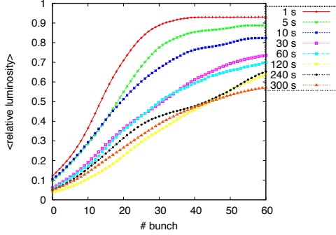
Figure 4: Beam-based IP position and IP angle feedback simulation for the e^+e^- collision with ground motion model B applied for successive time intervals along the BDS. The average relative luminosity is calculated over 50 seeds.
