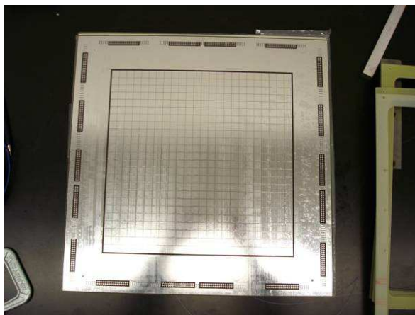
FIGURE 5.38. A 30 × 30 cm 2 GEM chamber prepared for test measurements. FE readout electronics is placed on the edge of the chamber frame.
