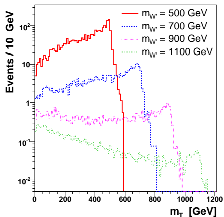
FIG. 1: Transverse mass m_T distributions for different masses of the W' boson (generator level, PYTHIA). The event numbers correspond to an integrated luminosity of 1 \text{ fb}^{-1} .
