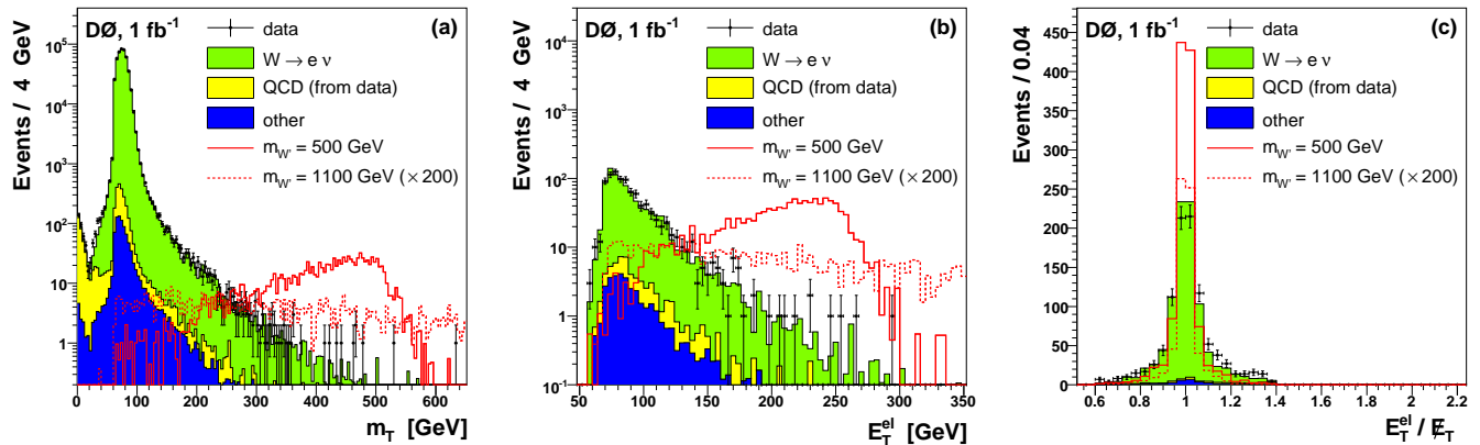
FIG. 2: Comparison between data and background prediction: (a) Distribution of the transverse mass m_T ; (b) distribution of the electron transverse energy E_T^{\text{el}} in events with m_T > 140 GeV; (c) distribution of the ratio of electron transverse energy and E_T in events with m_T > 140 GeV. The signal is shown for two different masses of the W' boson.
