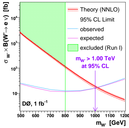
FIG. 3: The observed and expected 95% C.L. limits on the cross section as a function of the mass of the W' boson, including statistical and systematic uncertainties. The expected limit assumes a background-only hypothesis. The theoretical expectation is displayed with its uncertainty. Also shown is the D0 Run I limit [5].
