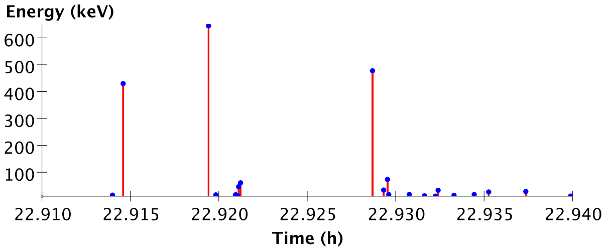
FIG. 4: Examples of event energies as a function of time. Some large events ( E > 300 keV) appear after relatively quiet periods (for instance just before 22.92 h) whereas others have some precursors (for instance just before 16.155 h) and others display aftershocks (around 22.93 h)
