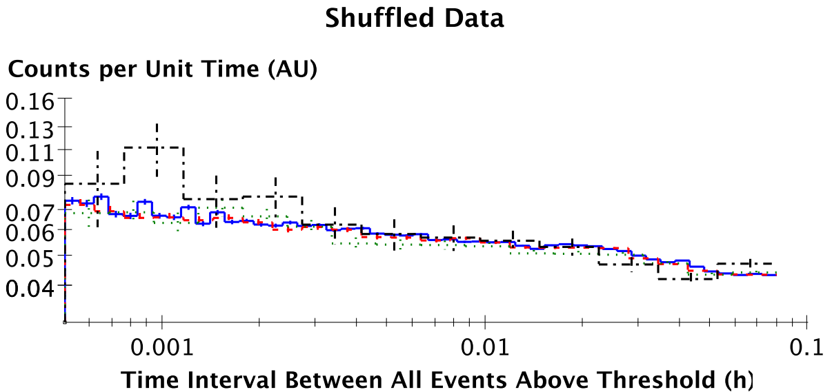
FIG. 3: Distribution of times between all (as opposed to consecutive) events in various energy ranges (note binning varies between ranges). Top: in the data, the distribution becomes peaked at low times as the event size increases. This is an indicator of clustering for large events. Bottom: in a random shuffle of the data, the distributions differ less for all event sizes.
