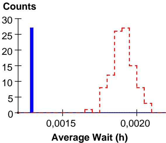
FIG. 5: Fig. A shows the average wait between a small (12–30 keV) event and the event of any size preceding it (solid blue bar), and the distribution of this average wait before small events in 100 shuffles of data (dashed red histogram). Fig. A' shows the same but for large events (300–1000 keV). Fig. A and A' demonstrate that there is significantly less wait on average before a large event than before a small one. However, Fig. B illustrates that though the averages differ, the distribution of waiting times before small and large events are quite similar and will not provide strong discrimination between individual small and large events. Fig. C shows the distribution of counts in random intervals (solid blue line), in intervals before small events (dashed red) and in intervals before large events (dotted green). The distributions do not show a strong distinction between small and large events, and indeed little difference between random intervals and intervals preceding events.
