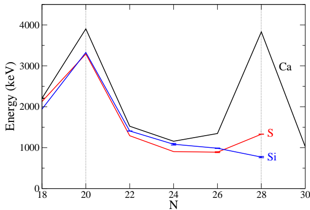
Fig. 3. Experimental E(2^+_1) values in the ^{14}\text{Si} , ^{16}\text{S} and ^{20}\text{Ca} isotopic chains as a function of the neutron number N . Data are taken from the compilation of Ref. 25 except for ^{38}\text{Si} , 26 ^{40}\text{Si} , 24 ^{42}\text{Si} , 3 and ^{40}\text{S} . 27
