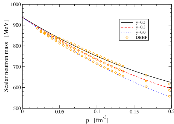
FIG. 3: (Color online) Comparison between the best RMF adjustment and the scalar mass calculated with DBHF approach. The asymmetry parameter y = \rho_p/\rho_B , ranges from 0.5 to 0. It clearly shows a linear ( f_\sigma^2 \rho_B ) and a quadratic ( f_\sigma^4 \rho_B^2 ) behavior in the baryonic density. The isospin asymmetry is also well reproduced by the linear term f_\delta^2 \rho_3 in the asymmetry density \rho_3 .
