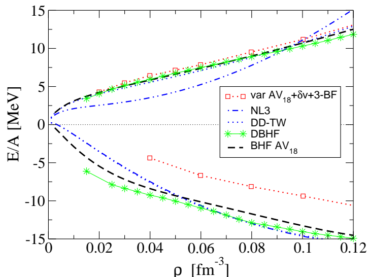
FIG. 1: (Color online) Comparison of several equation of state with the DBHF results. The DBHF calculation are represented by the stars, the variational by the empty squares, the non-relativistic Brueckner results by the dashed line and two different relativistic mean field parametrisations: NL3 (dashed-dotted line) and DD-TW (dotted line).
