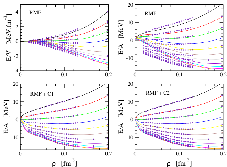
FIG. 4: (Color online) Comparison of the DBHF results (circles points) and the low density functionals in asymmetric nuclear matter. On the top panels are shown the energy density and the binding energy for the parameters RMF, while on the bottom panels are shown the binding energies for the corrected functionals RMF+C1 and RMF+C2.
