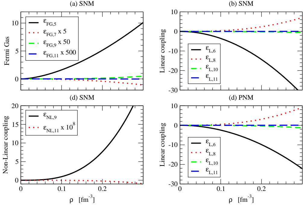
FIG. 2: (Color online) Representation of the different terms in the serie expansion of the energy functional with respect to the baryonic density, up to 0.3 \text{ fm}^{-3} . The first 3 subsets show the fast convergence in symmetric nuclear matter (SNM) and the last subset (d) show the contribution of the isovector mesons in pure neutron matter (PNM). To give an idea of the fast convergence, we have multiplied some of the terms by huge constants. The coupling constants (set A NL\rho\delta ) obtained by Liu et al. [42] has been used.
