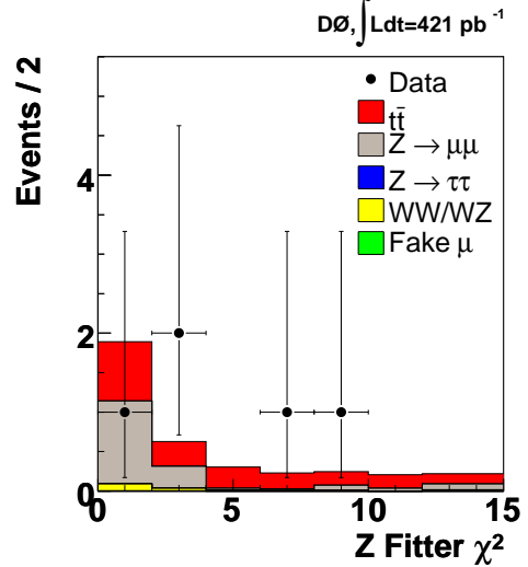
FIG. 7: The observed and predicted \chi^2 distributions of dimuon events before the \chi^2 cut.
