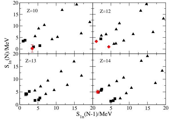
Figure 1. S_{1n}(N) as a function of S_{1n}(N-1) where N is the neutron number. The triangles are from the mass table [12], the diamonds and the squares represent the new and improved (respectively) results measured in the present work.
