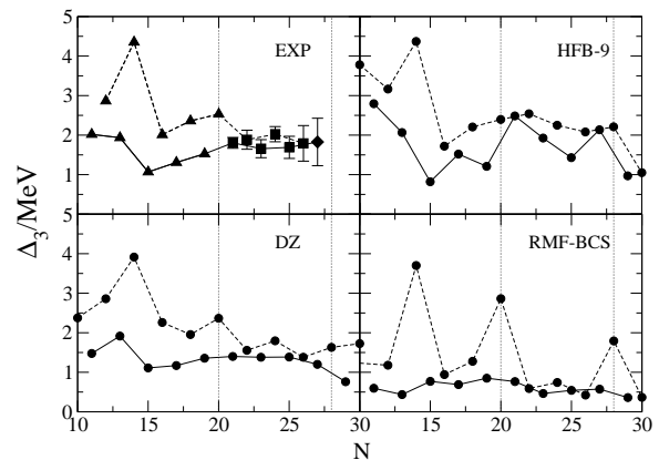
Figure 4. Experimental values of \Delta_3 for the Z=14 isotopic chain in comparison with three different mass formulas (see text). The vertical lines indicate the position of N=20 and 28 .
