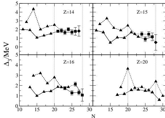
Figure 2. Experimental results for the three-point indicator \Delta_3 as function of neutron number. The same symbols are used as in figure 1. The dashed lines link the values of \Delta_3 for even- N nuclei and the full lines for odd- N nuclei. The vertical lines indicate the position of N=20 and 28.
