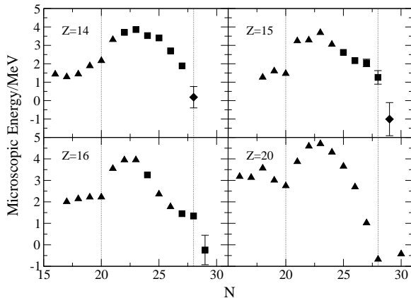
Figure 3. The microscopic correction as function of neutron number. The same symbols are used as in figure 1. The vertical lines indicate the position of N=20 and 28 .
