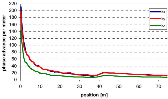
Figure 4 Full current phase advance per meter along the DTL-CCDTL-SCL.
