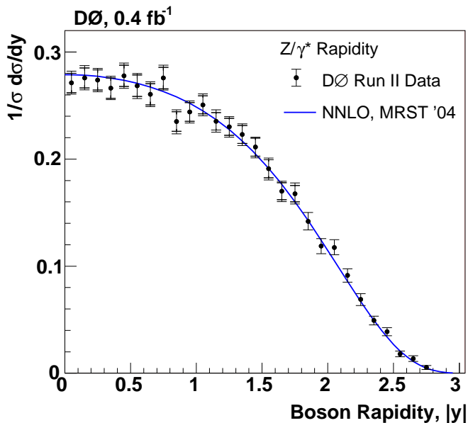
FIG. 4: DØ Run II measurement of \frac{1}{\sigma}d\sigma/dy vs |y| . The inner (outer) error bars show the statistical (total) uncertainty. The curve is a NNLO calculation from [1] using MRST 2004 PDFs.
