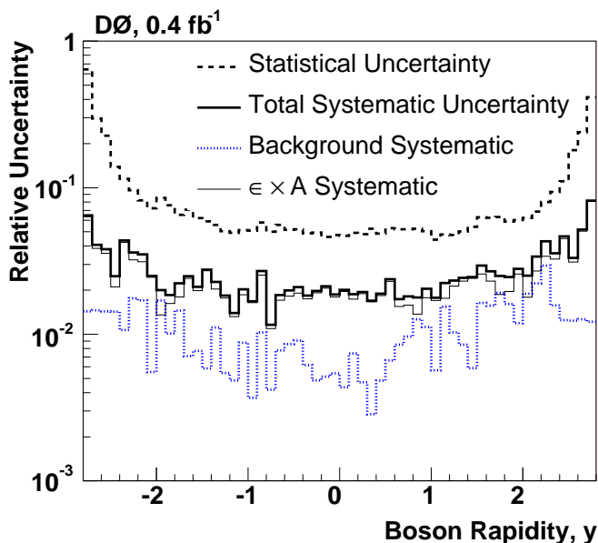
FIG. 2: Relative uncertainties plotted against the boson rapidity.
