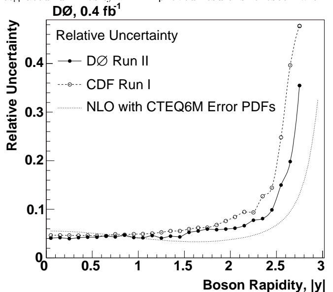
FIG. 5: Relative uncertainties from this measurement and from the CDF Run I result. Also shown is the PDF uncertainty on the differential cross section using the CTEQ6M uncertainty PDF sets. The values for the CTEQ6M curve are generated with code from Ref. [1].
