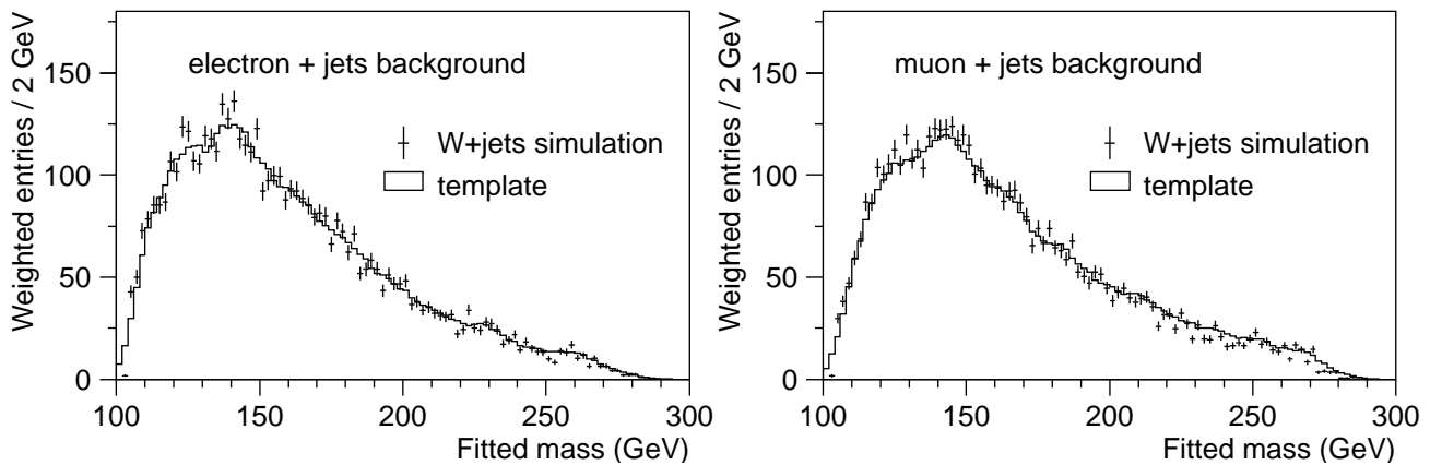
FIG. 2: Histograms showing the background shape from a weighted sum (see text) of all twenty-four masses from each event from the W +jets background sample (points with error bars), for the electron+jets channel (left) and muon+jets (right). The histograms show the shapes that are used in the likelihood. To reduce statistical fluctuations, the shapes are calculated as the average value in a sliding window of \pm 5 GeV around each fitted mass.
