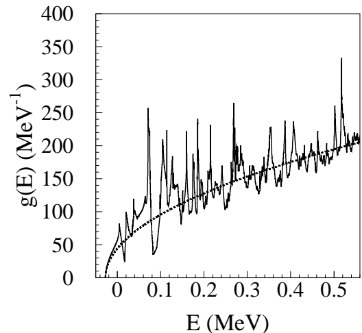
FIG. 5: Unbound single particle energy spectrum obtained in the W-S approximation.
