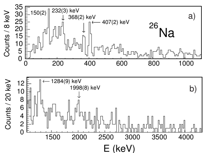
FIG. 11: Low-energy (a) and high-energy (b) part of the \gamma spectrum of ^{26}\text{Na} . The spectrum is Doppler corrected with a velocity \beta=0.095 . The neutron separation energy of ^{26}\text{Na} is S_n=5.576(6) MeV [38].
