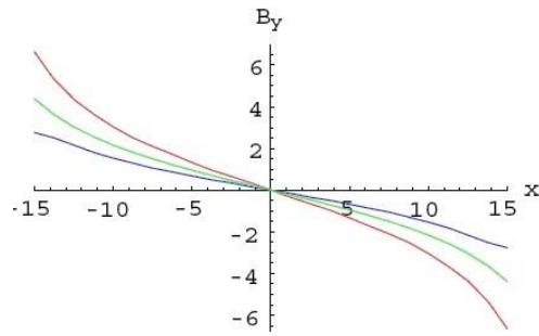
Figure 4: Sum of the fields produced by N pairs of conductors, with an interval of g (red), 1.3g (green) and 2g (dark blue). N decreases with increasing n .
