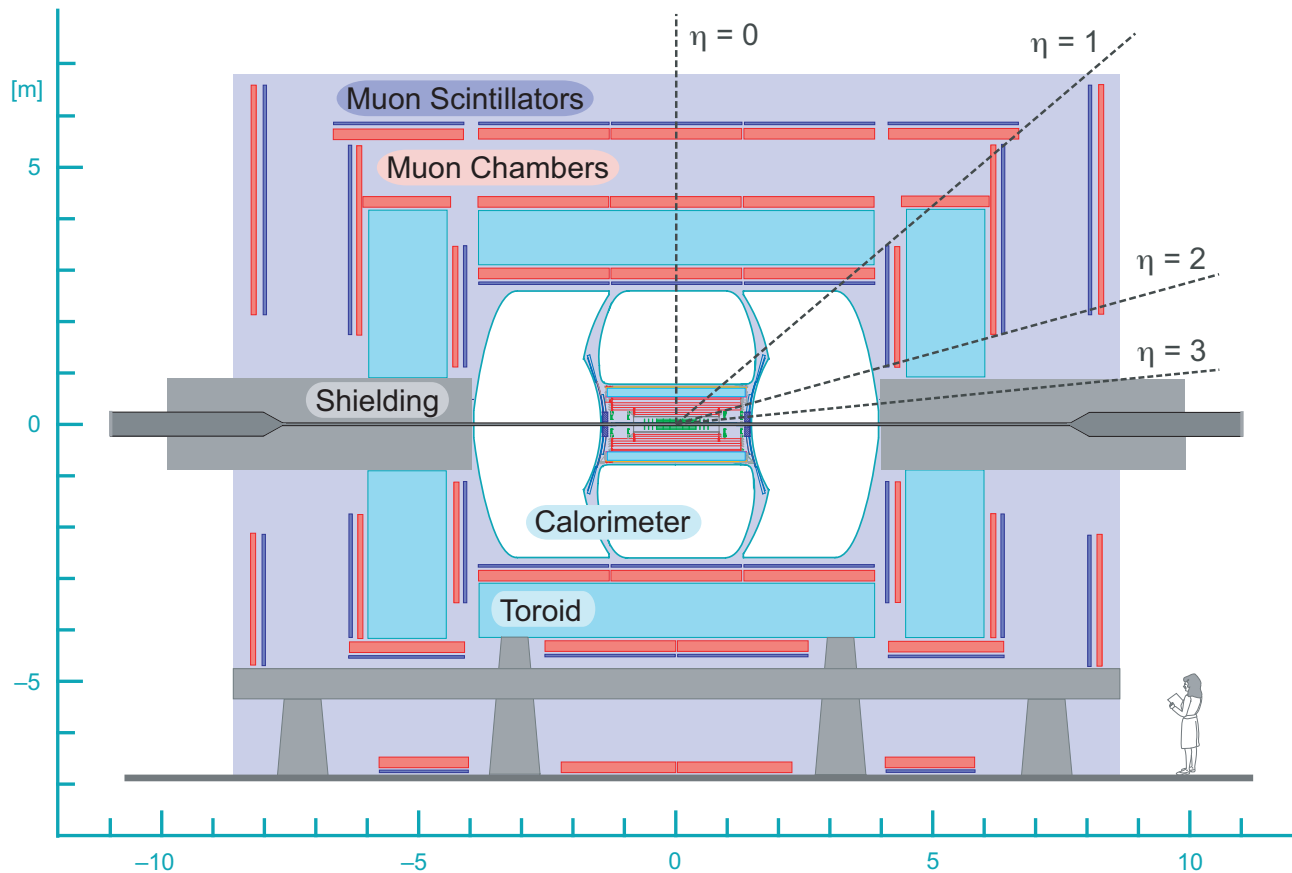
FIG. 5: General view of the D\bar{O} detector. The proton beam travels from left to right and the antiproton beam from right to left in this figure.
