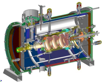
Figure 5: Cryomodule design for the SC-RF gun
