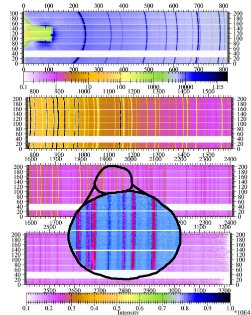
Fig. 5. Debye Scherrer reconstructed film
