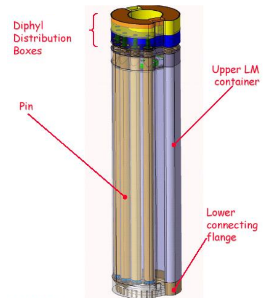
Figure 6 : View of the target heat exchanger with the upper liquid metal container.
