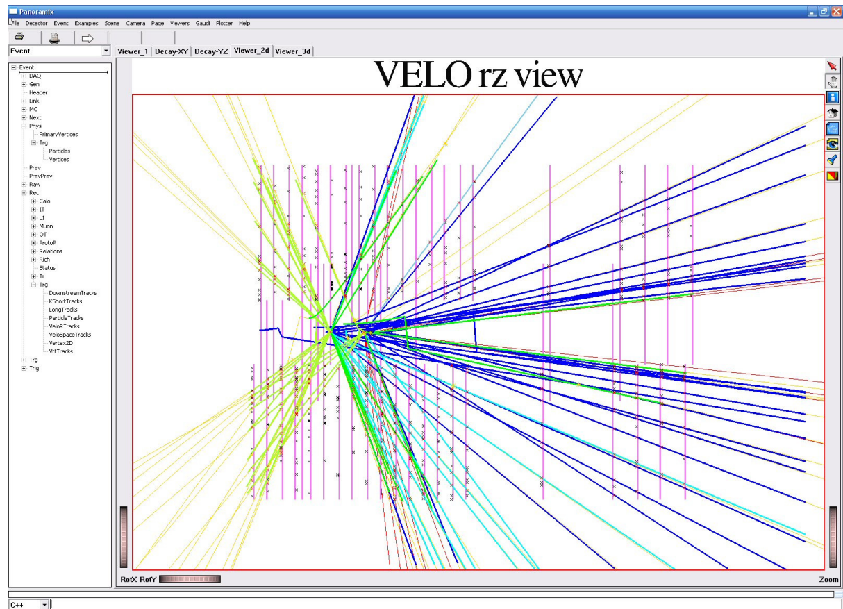
Figure 2-14: Close look at the interaction region showing the reconstructed tracks and their measurements in the Velo overlaid with the original Monte Carlo true tracks.
