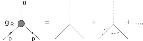
Figure 4. Renormalized coupling constant
