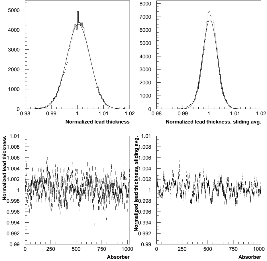
Fig. 10. Upper plots : Distribution of the normalized lead thickness for all the \eta cells of all the absorbers of the barrel calorimeter. The effect of optimizing the arrangement of consecutive absorbers can be seen in the reduction of the rms of the sliding average, 0.31% (right upper plot) instead of 0.44%. The thickness for each middle sampling cell is calculated by taking the average of all the measurements on the lead plate, that fall within the corresponding cell \eta range. From the r.m.s. of the distribution of the sliding average of the normalized thickness over 5 consecutive absorbers (upper right plot), it is possible to deduce that the contribution of the residual lead thickness inhomogeneities to the constant term [9] is 0.31\% \times 0.6 = 0.19\% . The normalized lead thickness as a function of \phi or absorber number shows that there are no systematic trends (lower plots).
