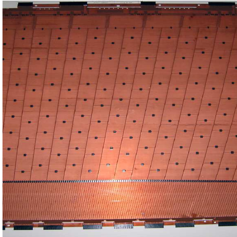
Fig. 7. Upper part: etched pattern, before folding, on A+B electrodes signal layer. Lower part: picture of a section, about 50 cm long, of an A electrode, before folding, showing the etched pattern of the HT layer where the resistive silk-screened pads of carbon-loaded epoxy ink can easily be seen. (The copper strips between connectors have not yet been removed.)
