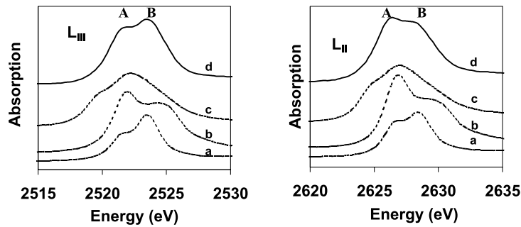
Fig. 9. XANES Mo L_{II,III} edge spectrum of (a) \text{Na}_2\text{MoO}_4 , (b) \text{MoO}_3 , (c) \text{MoO}_2 and (d) Mo implanted hydroxyapatite sample annealed at 300^\circ\text{C} for 5 h.
