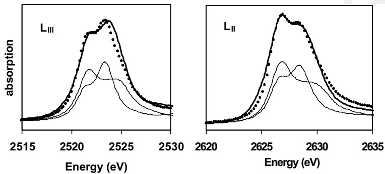
Fig. 10. XANES experimental spectrum (bold line) of 300^\circ\text{C} annealed sample modelled (dotted) by a mixture of 40% octahedral and 60% tetrahedral form (line).
