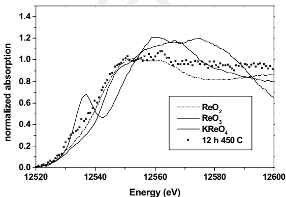
Fig. 11. Re L_I edge XANES spectra: comparison between reference compounds and a 450^\circ\text{C} annealed hydroxyapatite sample implanted in rhenium.
