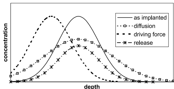
Fig. 1. Effect of diffusion, driving force towards the surface and matter release on the profile evolution of implanted species.
