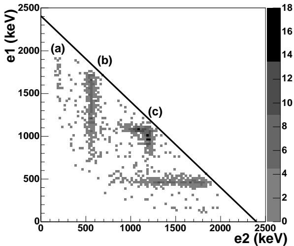
Fig. 6. The reconstructed two dimensional energy distribution of the experimental two-proton events. The y axis corresponds to the center of mass energy of the first transition, from one excited state in ^{19}\text{Na} to one excited state in ^{18}\text{Ne} , the x axis is the energy of the second transition from the state in ^{18}\text{Ne} to ^{17}\text{F}_{gs} . The continuous line corresponds to the maximum energy available in center of mass system. The 3 clusters of events producing the vertical lines labelled (a), (b) and (c), correspond to sequential transitions (see text).
