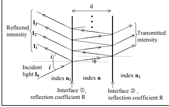
Fig. 1. a) Principle of the Fabry-Perot cavity.
