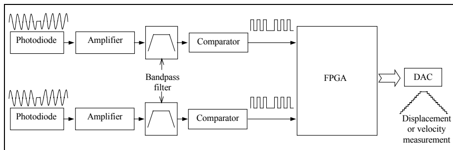
Fig.7. Simplified block diagram of the signal processing.
