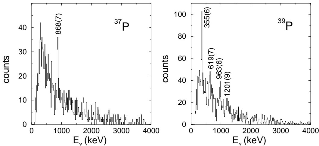
Fig. 2. Germanium \gamma -ray spectra of 37 P and 39 P nuclei produced in fragmentation of 48 Ca.
