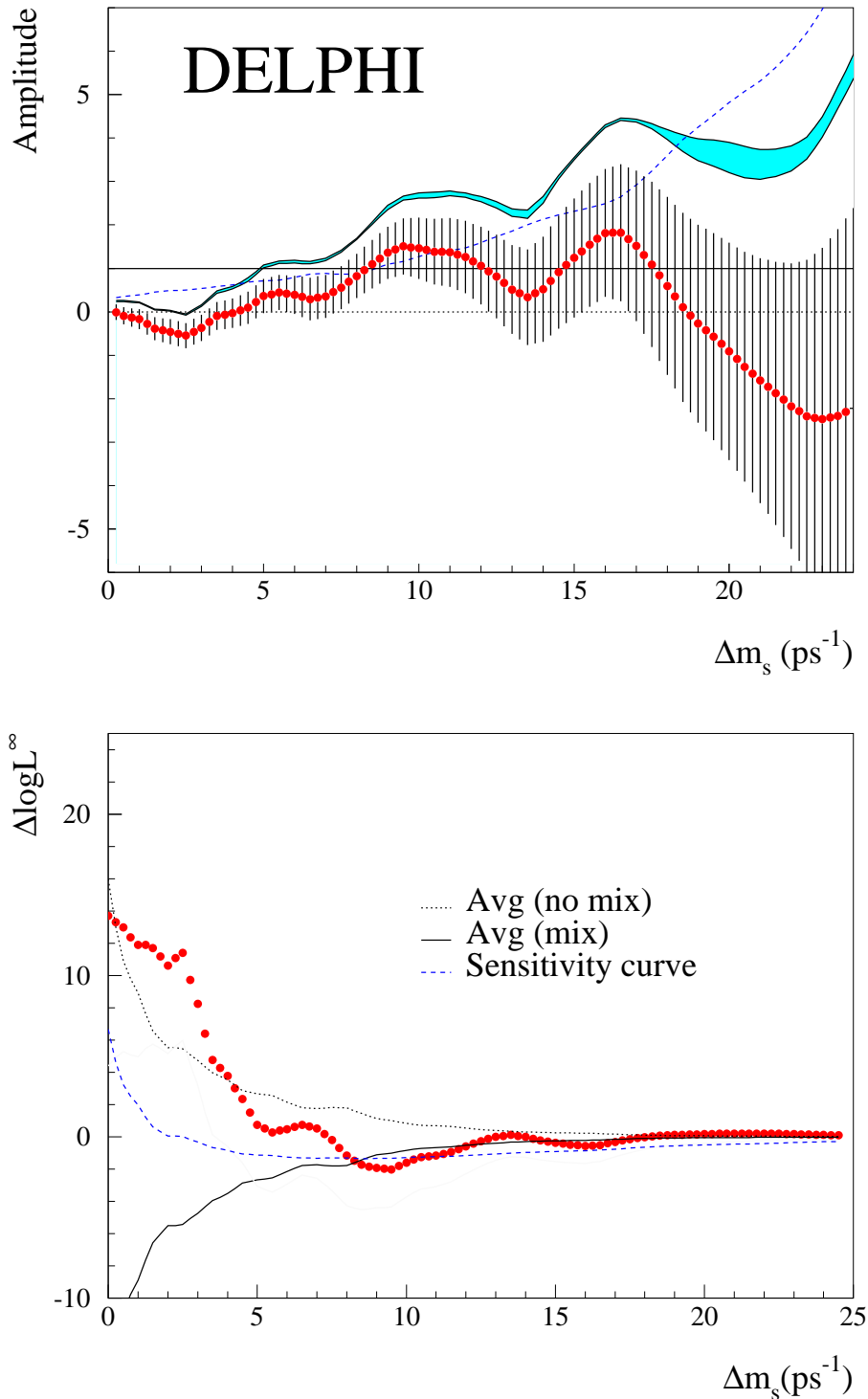
Figure 12: DELPHI D_s^\pm \ell^\mp analysis: the upper plot shows the variation of the oscillation amplitude \mathcal{A} as a function of \Delta m_s . The filled area shows the variation of the contour corresponding to \mathcal{A} + 1.645\sigma_{\mathcal{A}} when the systematic uncertainty is included. The dotted line shows the sensitivity. The likelihood referenced to \Delta m_s = \infty (lower plot), represented by points, has been deduced from the amplitude spectrum using the formula given in [10] (see section 3.2).
