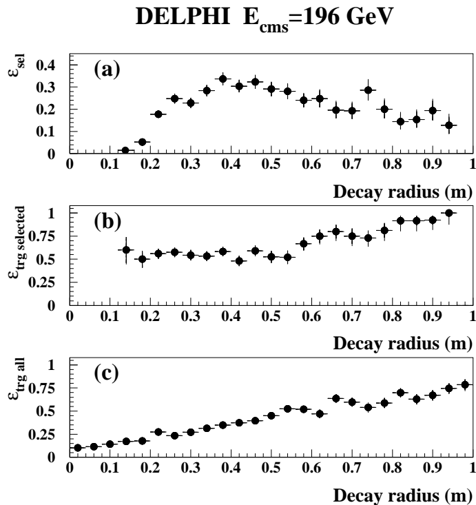
Figure 33: (a) Efficiency for selecting a single 75 \text{ GeV}/c^2 chargino in the search for displaced decay vertices (kinks) at the centre-of-mass energy of 196 \text{ GeV} , as function of its decay radius. (b) Trigger efficiency for the selected charginos. (c) Trigger efficiency for all 75 \text{ GeV}/c^2 charginos, whether or not they were selected.
