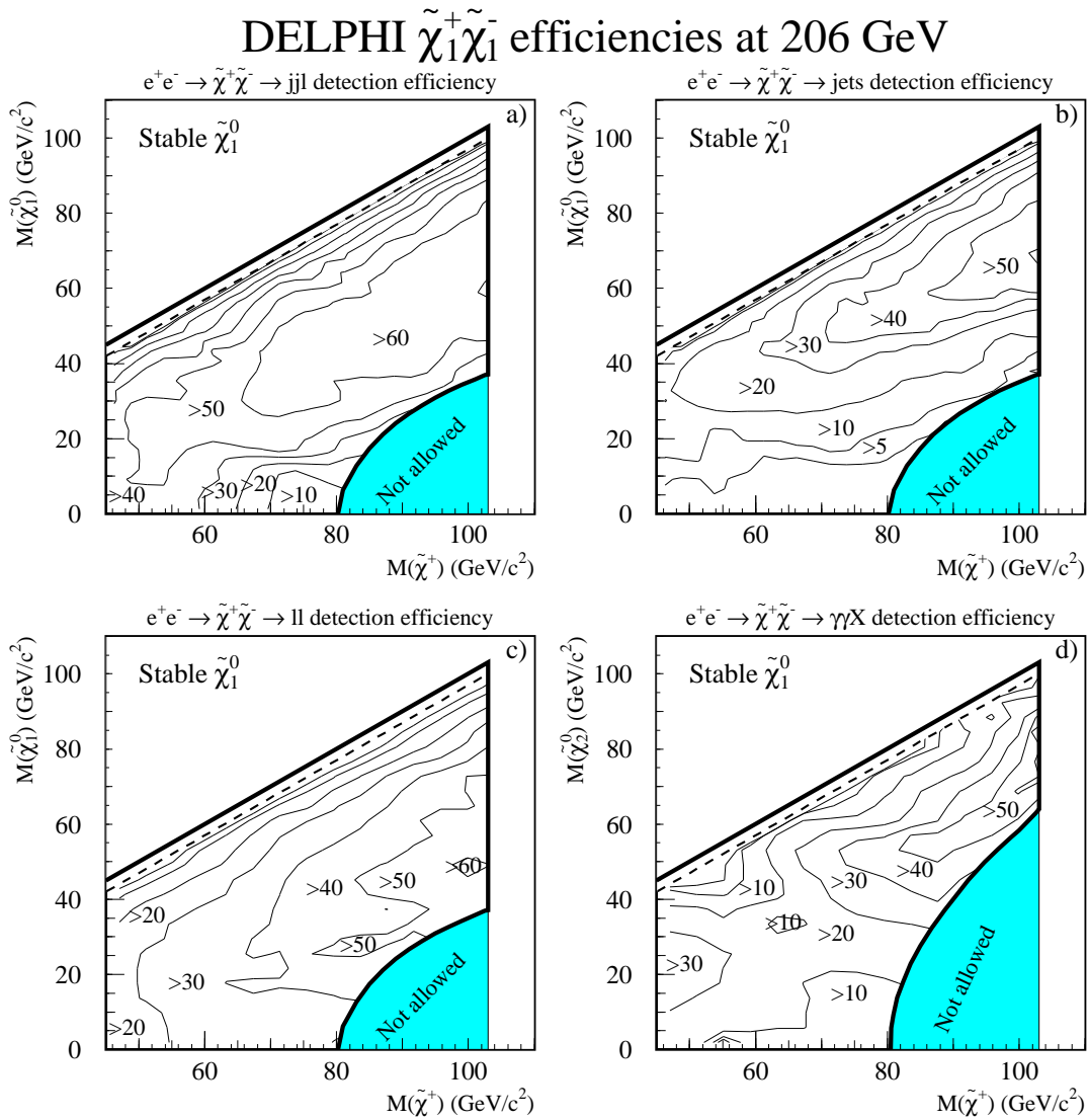
Figure 26: Chargino pair-production detection efficiencies (%) for the four decay channels a) jj\ell , b) \text{jets} , c) \ell\ell and d) \text{rad} , at 206 GeV in the (M_{\tilde{\chi}^\pm}, M_{\tilde{\chi}^0}) plane. TPC sector 6 is on and a stable \tilde{\chi}_1^0 is assumed. The shaded areas are disallowed in the MSSM scheme.
