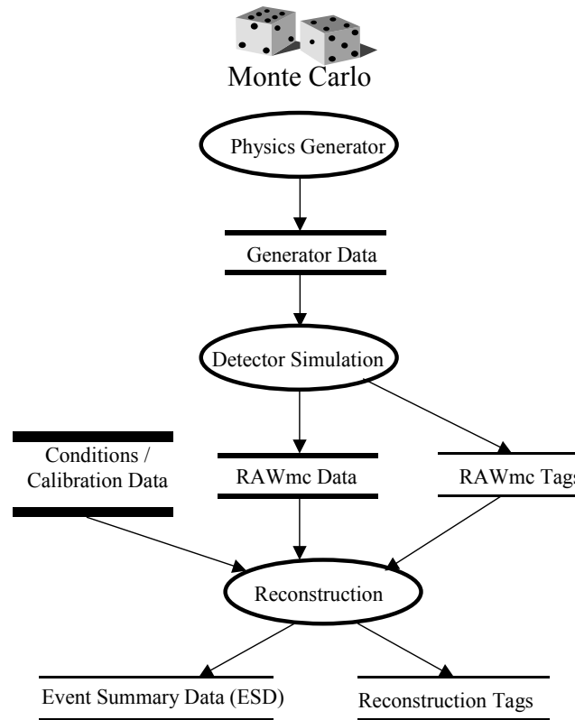
Fig. 1 The different steps of the Monte Carlo production
