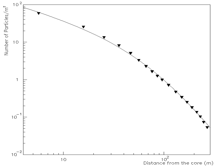
Fig. 2: Mean experimental lateral distribution of EAS, measured 2000 m a.s.l., for showers with N_e > 10^5 [7]. The line is the best fit to the NKG formula (2.5).
