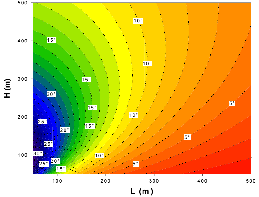
Fig. 14: The full FOV angle vs H and L. The diameter M of the imaged area has been fixed to 120 m.
