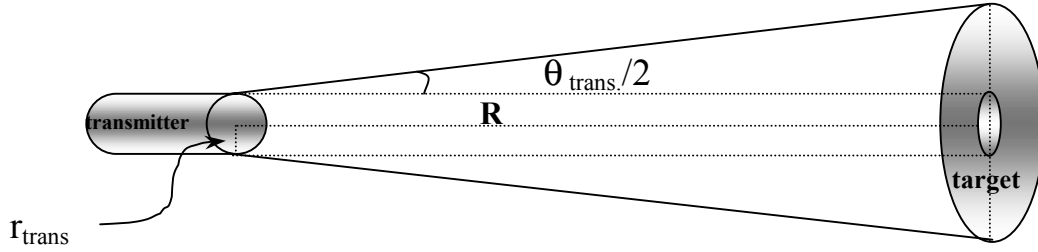
Fig. 21: Transmitter-target geometry.
