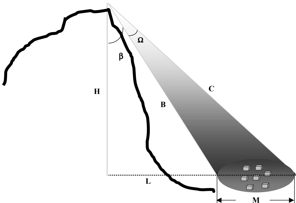
Fig. 12: Sketch of a typical configuration for the detection of Cherenkov light reflectively diffused by EAS. The gray ellipse represents graphically the coincidence area shared by the UVscope and ETscope array.
