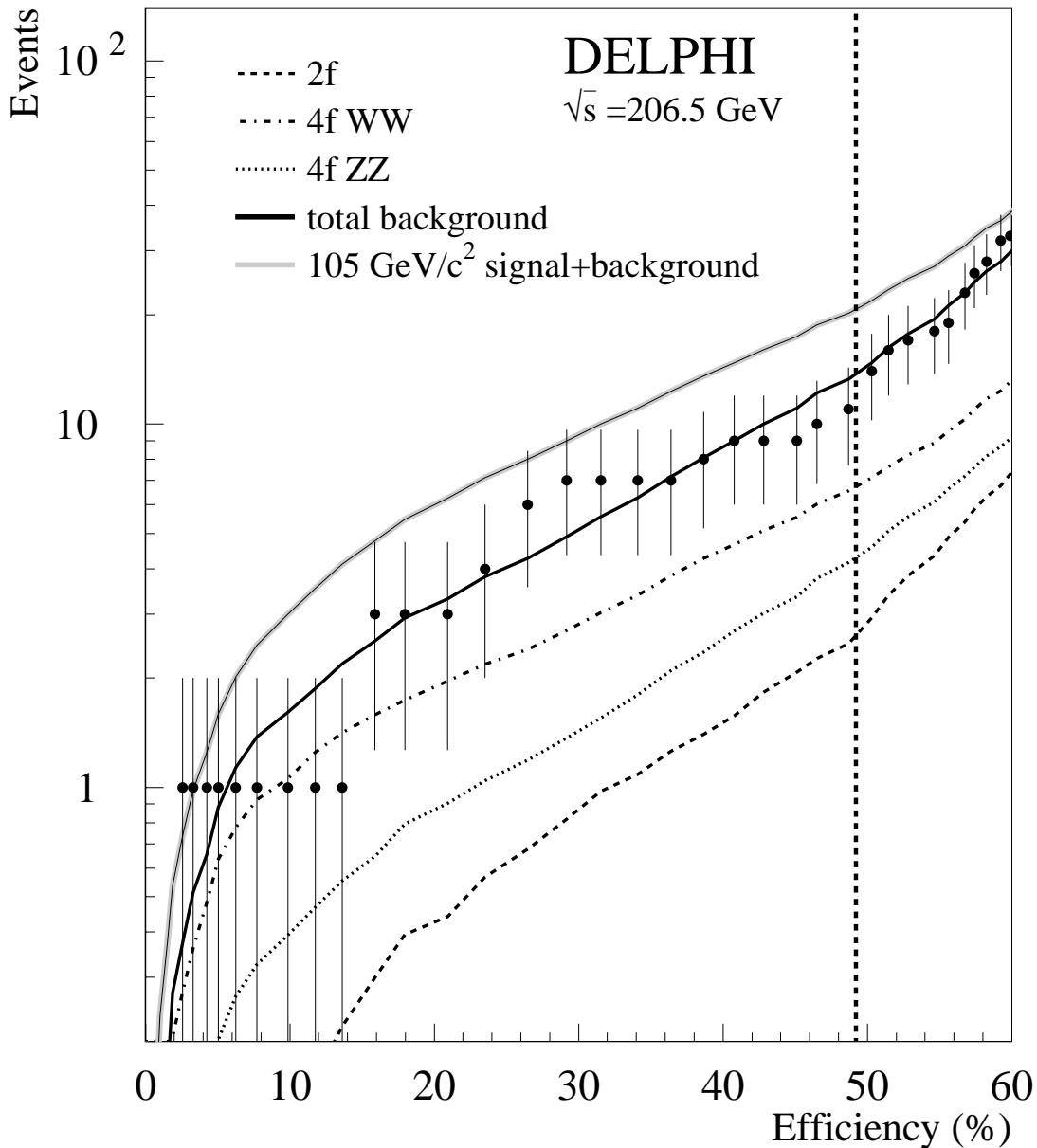
Figure 4: Hadronic channel high mass analysis: Data and expected background for the 206.5 GeV centre-of-mass energy as a function of the efficiency for an invisibly decaying Higgs boson of 105 GeV/c 2 . The lines represent the most important backgrounds with the solid black line showing the sum of all the background processes. In addition the grey line shows the expectation for a 105 GeV/c 2 Higgs signal added on top of the background. The vertical dashed line indicates the final cut chosen to maximise the sensitivity.
