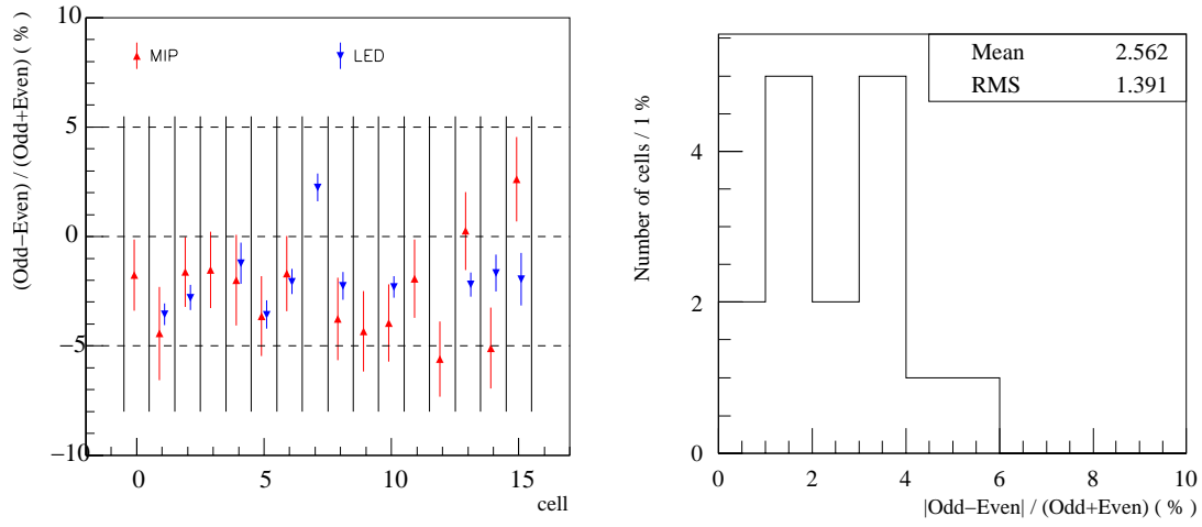
Figure 33: Left : half-channel gain relative differences for the 16 cells under study, as they were obtained from MIP and LED data. Right : distribution of the half-channel gain relative difference over the 16 cells of the PS module.
