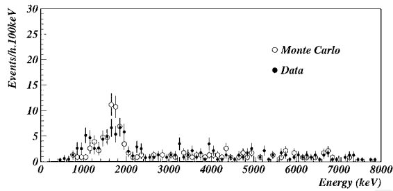
Fig. 6. Comparison of simulated and measured energy spectra of OCE events for 1 h with the Am-Be neutron source located on the east side of the NEMO 2 detector.
