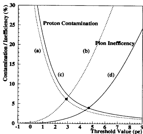
Fig. 8. \mathcal{P}(\pi \rightarrow P) and \mathcal{P}(P \rightarrow \pi) as a function of the threshold in photo-electrons. (a),(b) are for an average number of photo-electrons equal to 10.0 for \beta = 1 particles and (c),(d) are for an average number of 13.8
