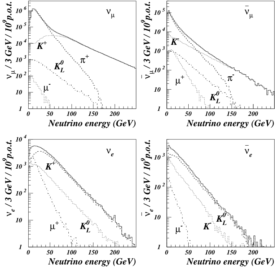
Figure 12: Composition of the \nu_\mu , \bar{\nu}_\mu , \nu_e and \bar{\nu}_e energy spectra at NOMAD, within the transverse fiducial area of 260 \times 260 \text{ cm}^2 .
