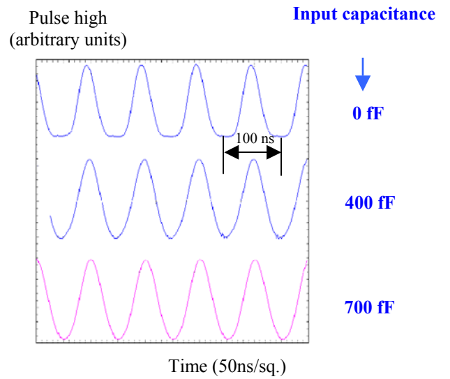
Fig. 5. Amplifier output with 10^7 pulse/sec, for three input capacitance's.
