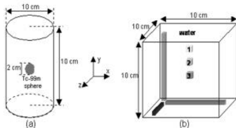
Fig. 1. Water cylinder (a) and water tank (b) phantoms.
