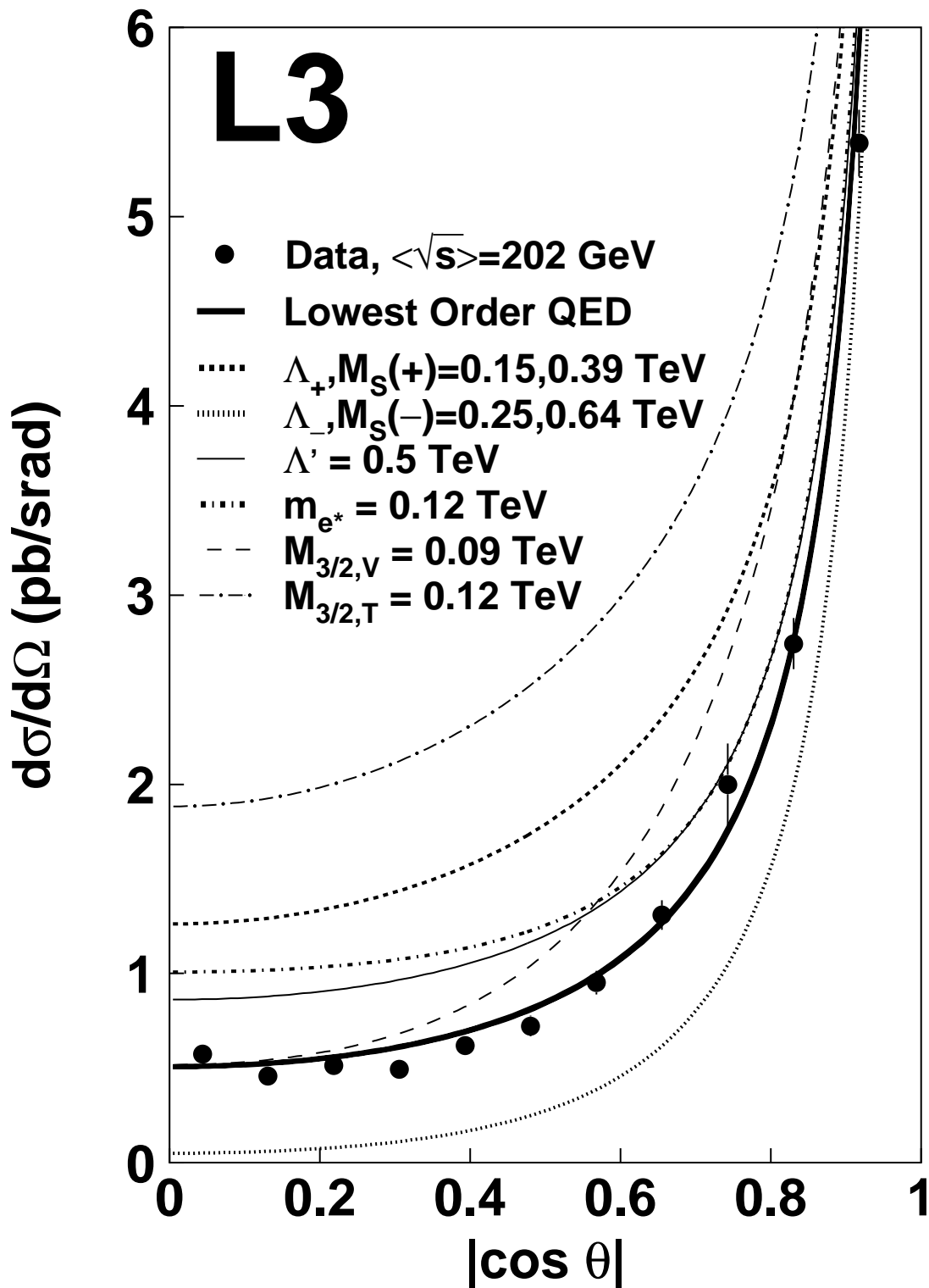
Figure 4: Differential cross sections as a function of \cos\theta . Points are data from \sqrt{s} = 192 to 208\text{ GeV} , corresponding to a luminosity weighted average of \langle\sqrt{s}\rangle = 202\text{ GeV} . Lines show the different predictions for the models discussed in the text at a centre-of-mass energy of \langle\sqrt{s}\rangle = 202\text{ GeV} . The width of the lowest order QED prediction takes into account the theoretical uncertainty, estimated to be 1%. The \chi^2 with respect to the QED prediction is 1.6 per degree of freedom.
