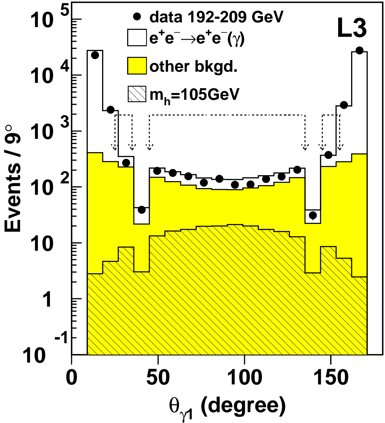
Figure 1: Distribution of the polar angle, \theta_{\gamma_1} of the most energetic photon for data and background. A Higgs boson signal with mass m_h = 105 GeV is superimposed with arbitrary normalisation. All Z final states are combined. The selected regions are indicated by the arrows.
