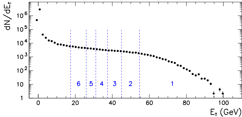
Figure 3: E_T in Pb–Pb collisions at 40 GeV per nucleon incident energy. The limits of the 6 centrality classes are superimposed.
