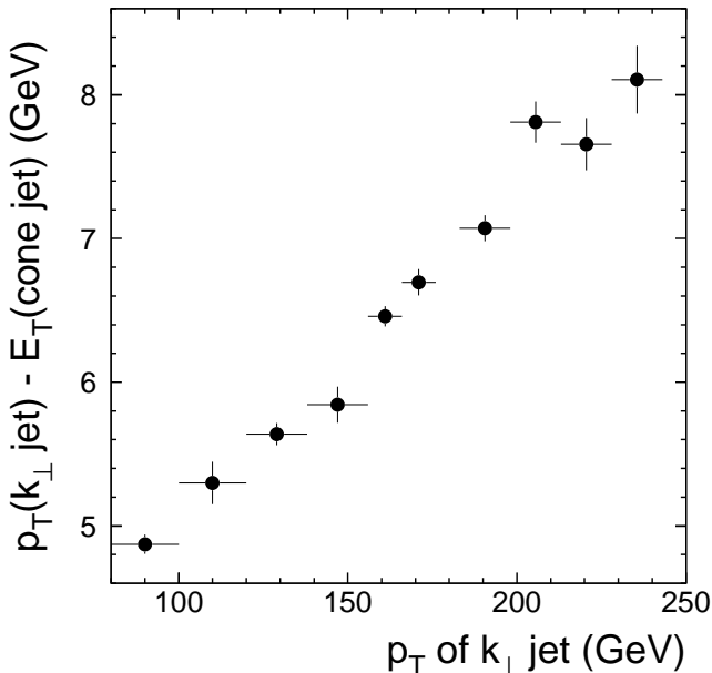
FIG. 11. The difference p_T(k_\perp \text{ jet}) - E_T(\text{cone jet}) as a function of the k_\perp jet p_T . A cone jet is associated with a k_\perp jet if their axes are separated by \Delta\mathcal{R} < 0.5 .
