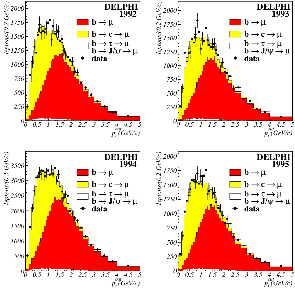
Figure 5: Comparison of the p_t^{out} distributions of prompt muons for the b flavour in real data (dots) with the distributions obtained using the semileptonic branching fractions (histograms). The contributions of different processes are displayed.
