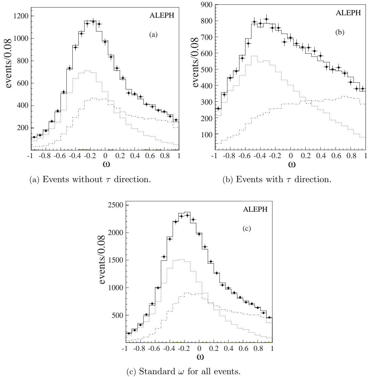
Figure 25: Distributions of the \omega observable used in the polarisation fit of the a_1 \rightarrow \pi^\pm 2\pi^0 channel. The data are shown by points with statistical errors bars. The dotted and dash-dotted lines corresponds to the contributions of left- and right-handed \tau 's respectively, as fitted in the data. The shaded area shows the non- \tau background contribution. The solid line corresponds to the sum of all simulated contributions.
