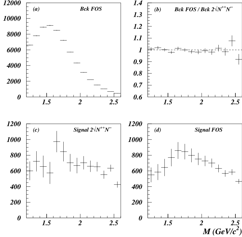
Figure 4: Comparison between the two background calculations, in the second centrality bin of Pb-Pb collisions. The FOS background is shown in (a). The ratio between FOS and 2\sqrt{N^{++}N^{--}} background, demonstrating the consistency between the two methods, is presented in (b). The signal spectra (c-d) are obtained by subtracting the combinatorial background spectra from the total opposite-sign dimuon mass distributions.
