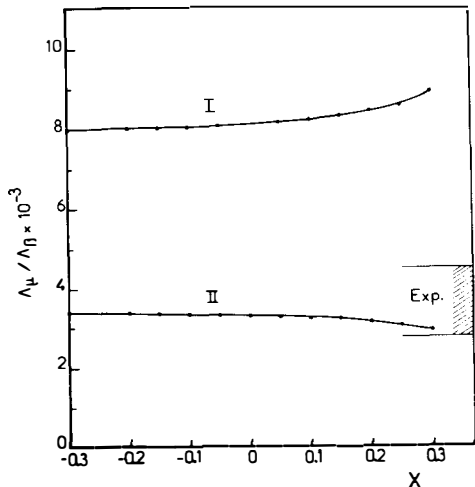
Fig. 1. Variation of the ratio \Lambda_\mu(0^+ \rightarrow 0^-)/\Lambda_\beta(0^- \rightarrow 0^+) versus configuration mixing coefficient X for the (1p_{3/2}^{-1}, 1d_{3/2}) component. The curve I corresponds to the impulse approximation, the curve II includes the mesonic exchange correction. The experimental ratio (Exp.) was evaluated from the Saclay muon capture experiment [10] ( \Lambda_\mu(0^+ \rightarrow 0^-) = 1570 \pm 100 \text{ s}^{-1} ) and from the Louvain \beta -decay experiment [11] ( \Lambda_\beta(0^- \rightarrow 0^+) = 0.43 \pm 0.10 \text{ s}^{-1} ).
